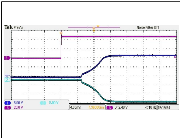
Figure 101: AEE01BB48-M Output Voltage Startup Characteristic by Vin Vin = 48Vdc Load: Io = ±0.625A Ta = 25°C Ch 1: Vo1 Ch 2: Vo2 Ch 3: Vin
