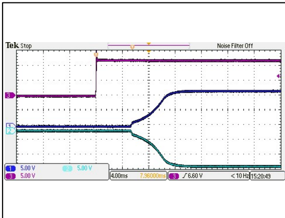
Figure 29: AEE01BB12-M Output Voltage Startup Characteristic by Vin Vin = 12Vdc Load: Io = ±0.625A Ta = 25°C Ch 1: Vo1 Ch 2: Vo2 Ch 3: Vin
