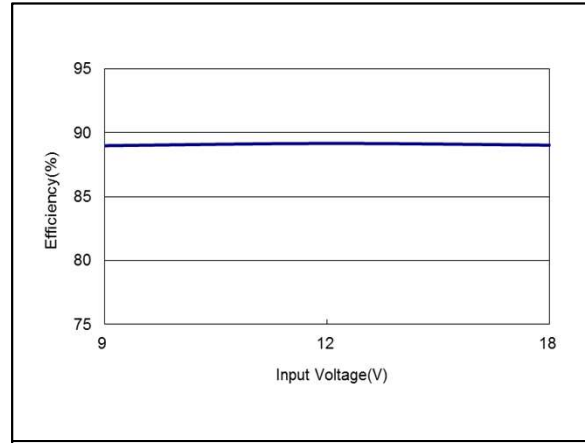
Figure 14: AEE01C12-M Efficiency Versus Input Voltage Curve Vin = 9 to 18Vdc Load: Io = 1A Ta = 25°C
