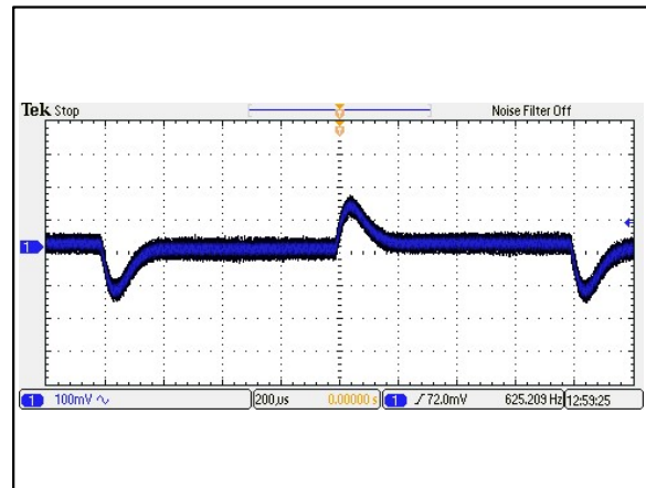
Figure 16: AEE01C12-M Transient Response Vin = 12Vdc Load: Io = 100% to 75% load change Ta = 25°C Ch 1: Vo
