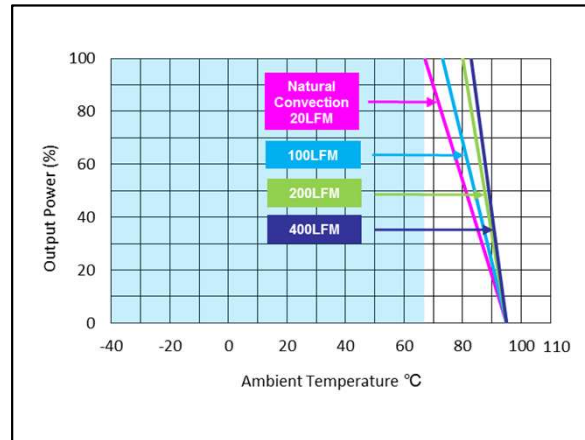
Figure 30: AEE01BB12-M Derating Curve (without heatsink). Vin = 12Vdc Load: Io = 0 to ±0.625A Ta = 25°C
