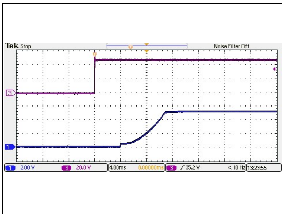
Figure 77: AEE03A48-M Output Voltage Startup Characteristic by Vin Vin = 48Vdc Load: Io = 3A Ta = 25°C Ch 1: Vo Ch 3: Vin
