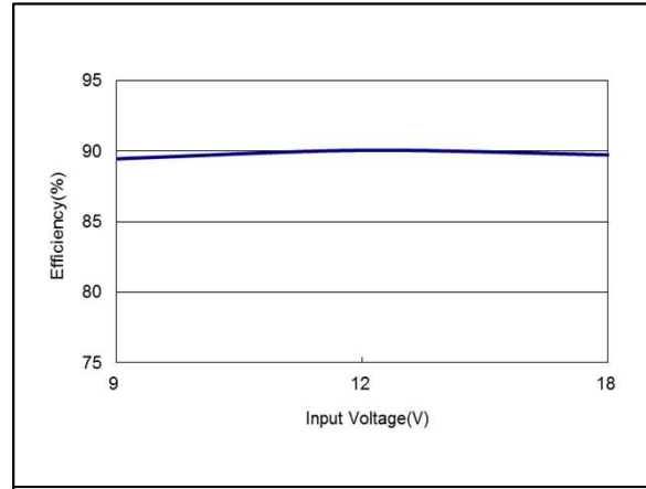
Figure 20: AEE01H12-M Efficiency Versus Input Voltage Curve Vin = 9 to 18Vdc Load: Io = 0.625A Ta = 25°C
