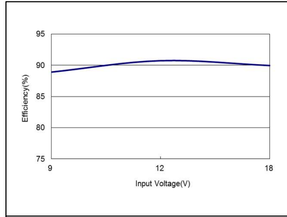
Figure 32: AEE01CC12-M Efficiency Versus Input Voltage Curve Vin = 9 to 18Vdc Load: Io = ±0.5A Ta = 25°C
