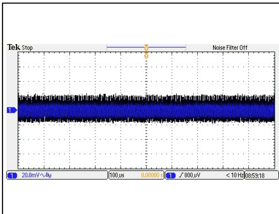
Figure 45: AEE01B24-M Ripple and Noise Measurement Vin = 24Vdc Load: Io = 1.25A Ta = 25°C Ch 1: Vo
