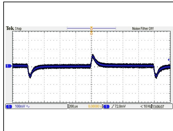
Figure 22: AEE01H12-M Transient Response Vin = 12Vdc Load: Io = 100% to 75% load change Ta = 25°C Ch 1: Vo
