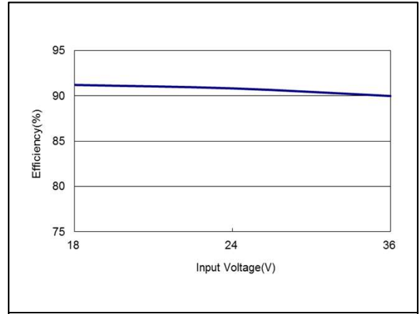
Figure 44: AEE01B24-M Efficiency Versus Input Voltage Curve Vin = 18 to 36Vdc Load: Io = 1.25A Ta = 25°C
