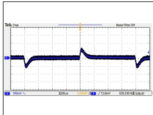
Figure 58: AEE01H24-M Transient Response Vin = 24Vdc Load: Io = 100% to 75% load change Ta = 25°C Ch 1: Vo
