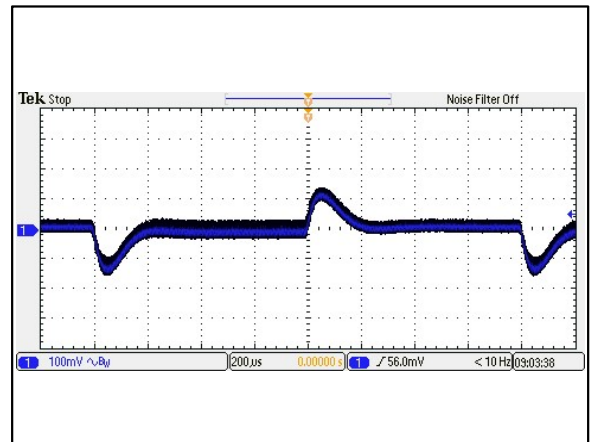
Figure 82: AEE01B48-M Transient Response Vin = 48Vdc Load: Io = 100% to 75% load change Ta = 25°C Ch 1: Vo
