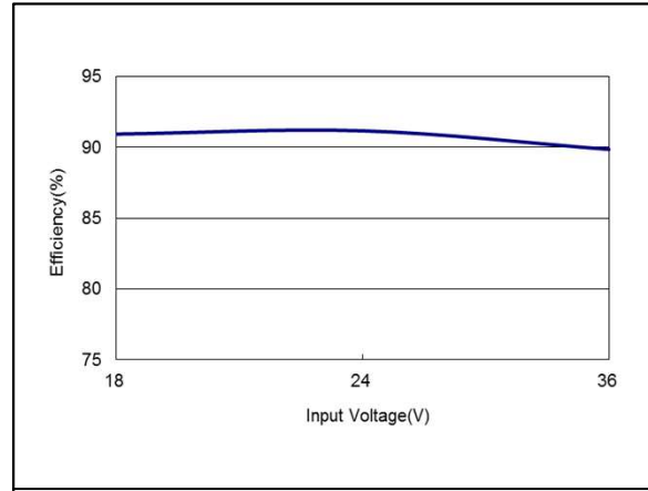
Figure 68: AEE01CC24-M Efficiency Versus Input Voltage Curve Vin = 18 to 36Vdc Load: Io = ±0.5A Ta = 25°C
