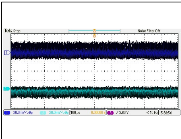
Figure 63: AEE01BB24-M Ripple and Noise Measurement Vin = 24Vdc Load: Io = ±0.625A Ta = 25°C Ch 1: Vo1 Ch 2: Vo2
