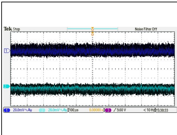
Figure 27: AEE01BB12-M Ripple and Noise Measurement Vin = 12Vdc Load: Io = ±0.625A Ta = 25°C Ch 1: Vo1 Ch 2: Vo2
