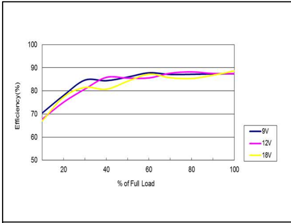
Figure 1: AEE03A12-M Efficiency Versus Output Current Curve Vin = 9 to 18Vdc Load: Io = 0 to 3A Ta = 25°C
