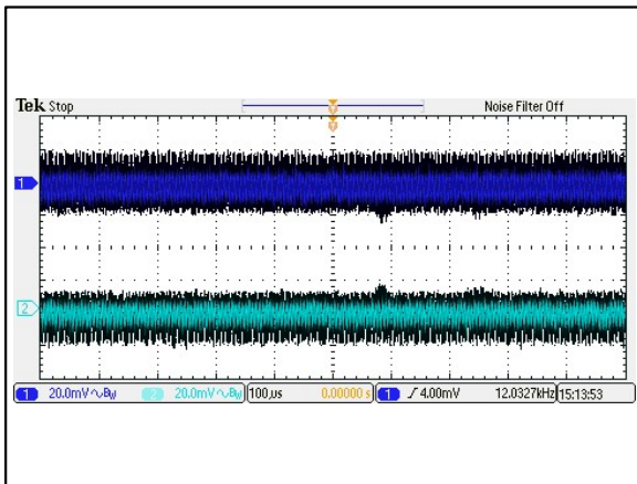
Figure 33: AEE01CC12-M Ripple and Noise Measurement Vin = 12Vdc Load: Io = ±0.5A Ta = 25°C Ch 1: Vo1 Ch 2: Vo2
