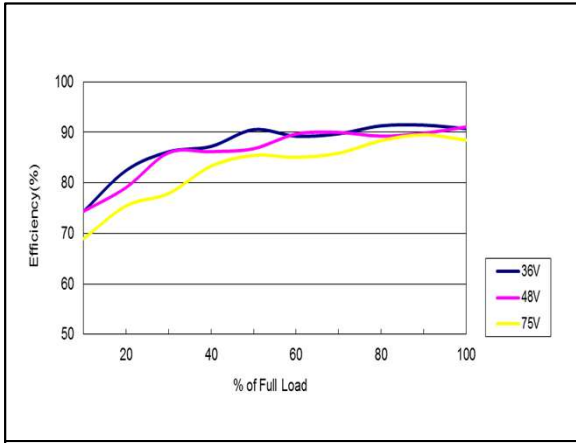
Figure 97: AEE01BB48-M Efficiency Versus Output Current Curve Vin = 36 to 75Vdc Load: Io = 0 to ±0.625A Ta = 25°C
