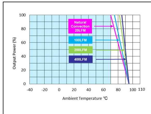
Figure 96: AEE01H48-M Derating Curve (without heatsink). Vin = 48Vdc Load: Io = 0 to 0.625A Ta = 25°C
