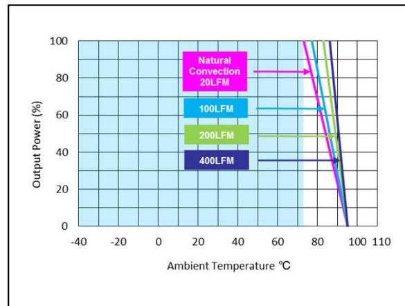
Figure 90: AEE01C48-M Derating Curve (without heatsink). Vin = 48Vdc Load: Io = 0 to 1A Ta = 25°C
