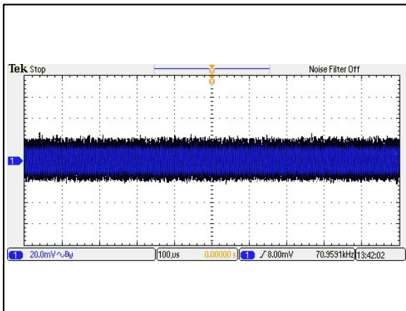
Figure 39: AEE03A24-M Ripple and Noise Measurement Vin = 24Vdc Load: Io = 3A Ta = 25°C Ch 1: Vo
