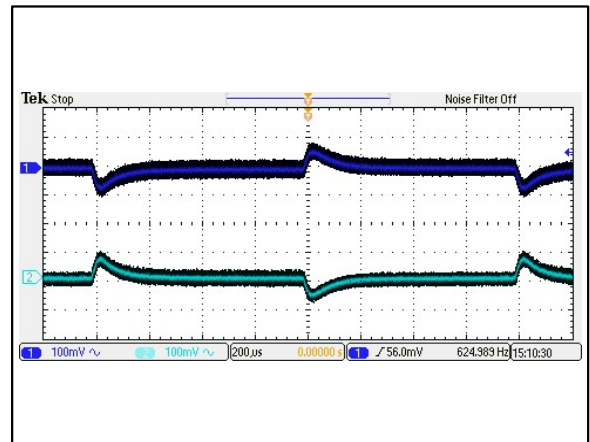
Figure 100: AEE01BB48-M Transient Response Vin = 48Vdc Load: Io = 100% to 75% load change Ta = 25°C Ch 1: Vo1 Ch 2: Vo2
