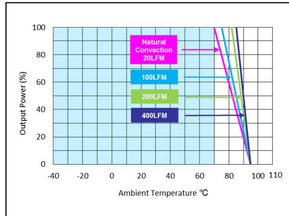
Figure 36: AEE01CC12-M Derating Curve (without heatsink). Vin = 12Vdc Load: Io = 0 to ±0.5A Ta = 25°C
