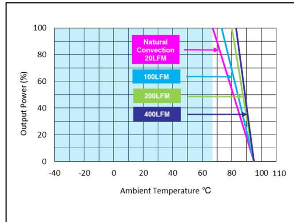
Figure 18: AEE01C12-M Derating Curve (without heatsink). Vin = 12Vdc Load: Io = 0 to 1A Ta = 25°C
