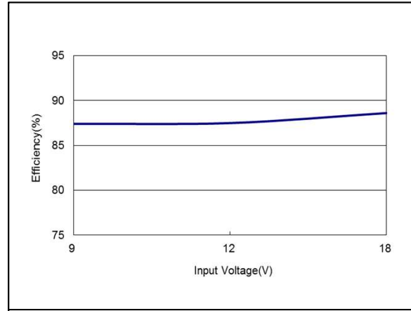
Figure 2: AEE03A12-M Efficiency Versus Input Voltage Curve Vin = 9 to 18Vdc Load: Io = 3A Ta = 25°C
