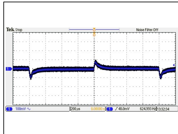
Figure 4: AEE03A12-M Transient Response Vin = 12Vdc Load: Io = 100% to 75% load change Ta = 25°C Ch 1: Vo
