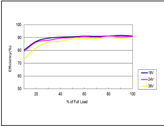
Figure 43: AEE01B24-M Efficiency Versus Output Current Curve Vin = 18 to 36Vdc Load: Io = 0 to 1.25A Ta = 25°C
