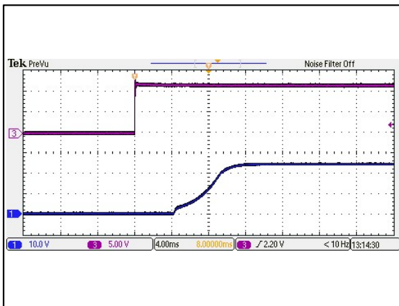
Figure 23: AEE01H12-M Output Voltage Startup Characteristic by Vin Vin = 12Vdc Load: Io = 0.625A Ta = 25°C Ch 1: Vo Ch 3: Vin
