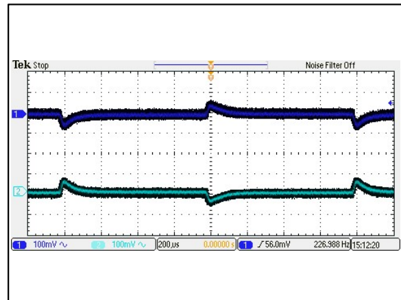
Figure 34: AEE01CC12-M Transient Response Vin = 12Vdc Load: Io = 100% to 75% load change Ta = 25°C Ch 1: Vo1 Ch 2: Vo2
