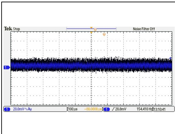
Figure 57: AEE01H24-M Ripple and Noise Measurement Vin = 24Vdc Load: Io = 0.625A Ta = 25°C Ch 1: Vo
