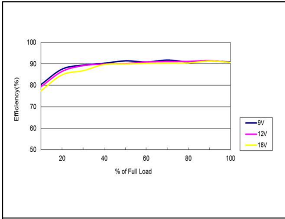
Figure 7: AEE01B12-M Efficiency Versus Output Current Curve Vin = 9 to 18Vdc Load: Io = 0 to 1.25A Ta = 25°C
