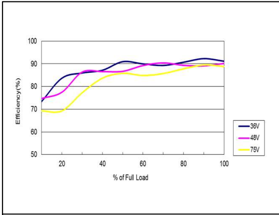
Figure 91: AEE01H48-M Efficiency Versus Output Current Curve Vin = 36 to 75Vdc Load: Io = 0 to 0.625A Ta = 25°C
