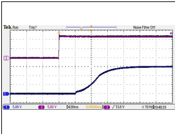
Figure 17: AEE01C12-M Output Voltage Startup Characteristic by Vin Vin = 12Vdc Load: Io = 1A Ta = 25°C Ch 1: Vo Ch 3: Vin
