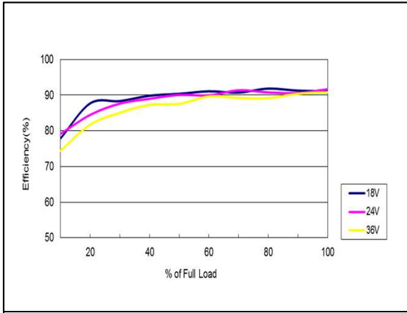
Figure 61: AEE01BB24-M Efficiency Versus Output Current Curve Vin = 18 to 36Vdc Load: Io = 0 to ±0.625A Ta = 25°C
