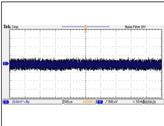
Figure 9: AEE01B12-M Ripple and Noise Measurement Vin = 12Vdc Load: Io = 1.25A Ta = 25°C Ch 1: Vo
