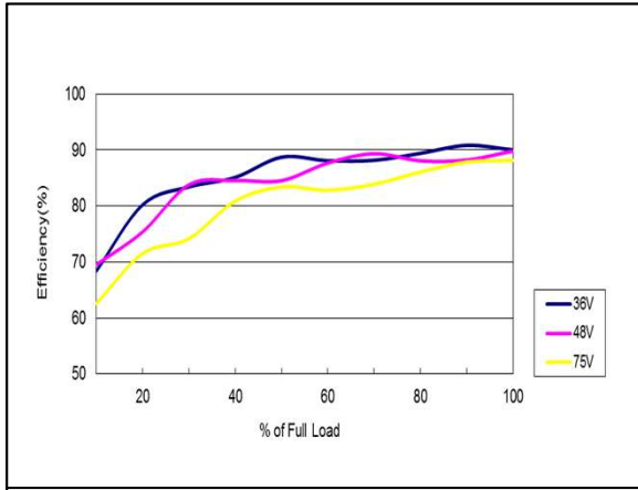
Figure 103: AEE01CC48-M Efficiency Versus Output Current Curve Vin = 36 to 75Vdc Load: Io = 0 to ±0.5A Ta = 25°C
