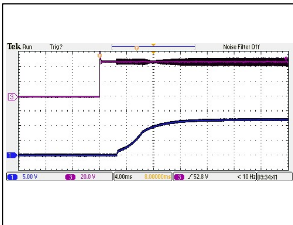
Figure 83: AEE01B48-M Output Voltage Startup Characteristic by Vin Vin = 48Vdc Load: Io = 1.25A Ta = 25°C Ch 1: Vo Ch 3: Vin
