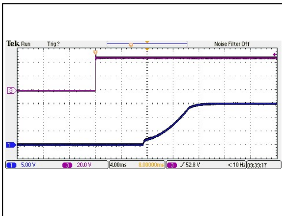
Figure 89: AEE01C48-M Output Voltage Startup Characteristic by Vin Vin = 48Vdc Load: Io = 1A Ta = 25°C Ch 1: Vo Ch 3: Vin
