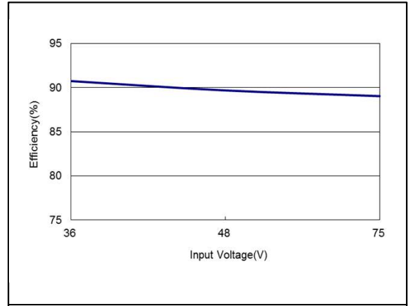
Figure 80: AEE01B48-M Efficiency Versus Input Voltage Curve Vin = 36 to 75Vdc Load: Io = 1.25A Ta = 25°C
