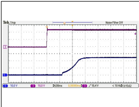
Figure 59: AEE01H24-M Output Voltage Startup Characteristic by Vin Vin = 24Vdc Load: Io = 0.625A Ta = 25°C Ch 1: Vo Ch 3: Vin
