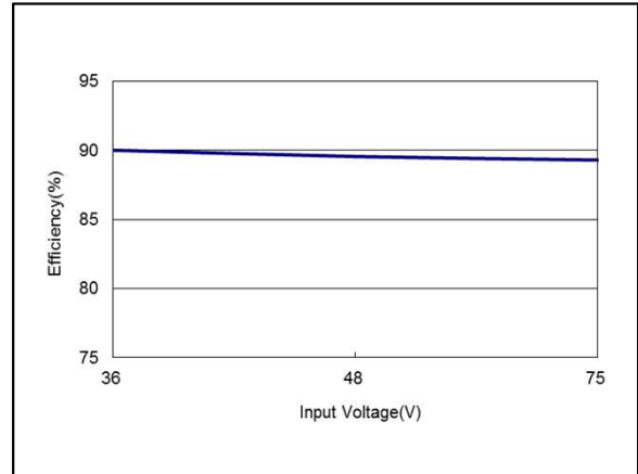
Figure 74: AEE03A48-M Efficiency Versus Input Voltage Curve Vin = 36 to 75Vdc Load: Io = 3A Ta = 25°C
