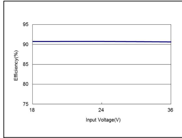
Figure 56: AEE01H24-M Efficiency Versus Input Voltage Curve Vin = 18 to 36Vdc Load: Io = 0.625A Ta = 25°C
