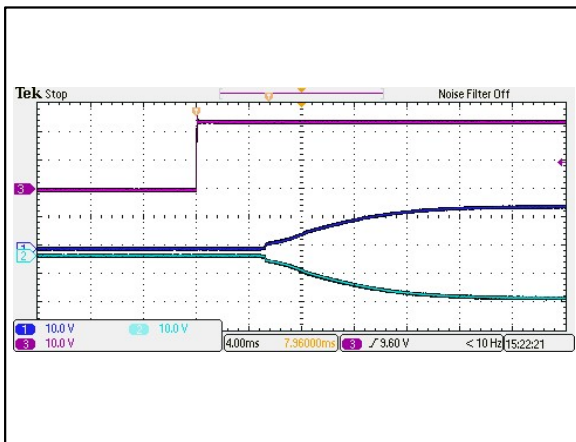
Figure 71: AEE01CC24-M Output Voltage Startup Characteristic by Vin Vin = 24Vdc Load: Io = ±0.5A Ta = 25°C Ch 1: Vo1 Ch 2: Vo2 Ch 3: Vin
