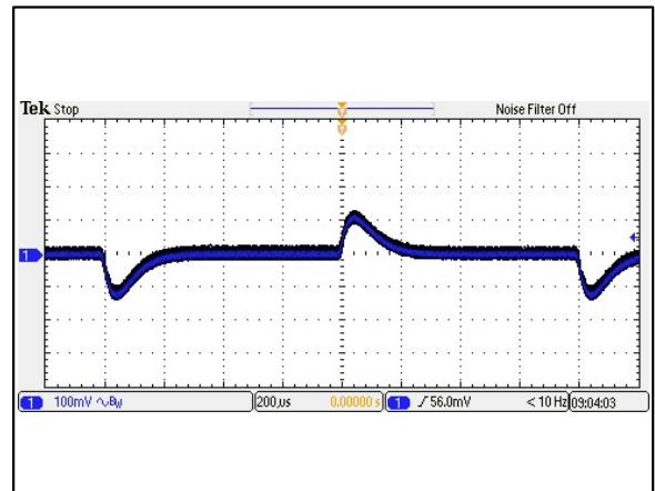
Figure 46: AEE01B24-M Transient Response Vin = 24Vdc Load: Io = 100% to 75% load change Ta = 25°C Ch 1: Vo
