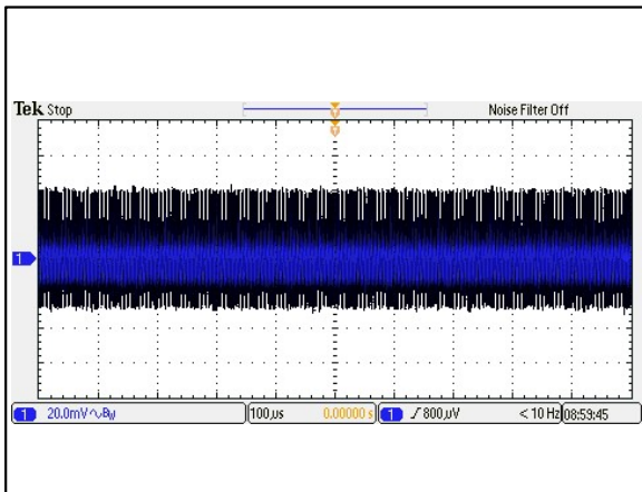
Figure 81: AEE01B48-M Ripple and Noise Measurement Vin = 48Vdc Load: Io = 1.25A Ta = 25°C Ch 1: Vo
