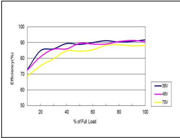
Figure 85: AEE01C48-M Efficiency Versus Output Current Curve Vin = 36 to 75Vdc Load: Io = 0 to 1A Ta = 25°C
