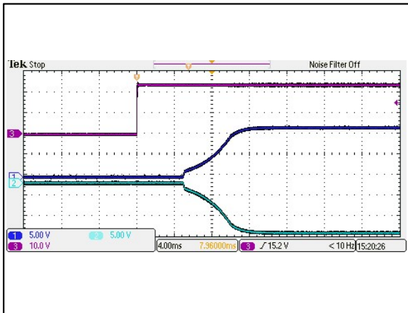
Figure 65: AEE01BB24-M Output Voltage Startup Characteristic by Vin Vin = 24Vdc Load: Io = ±0.625A Ta = 25°C Ch 1: Vo1 Ch 2: Vo2 Ch 3: Vin
