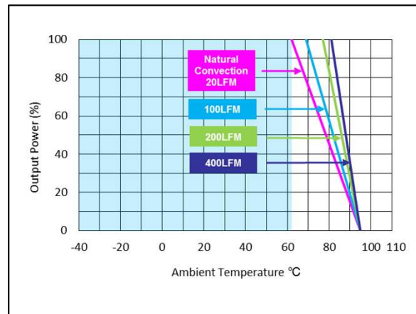
Figure 6: AEE03A12-M Derating Curve (without heatsink). Vin = 12Vdc Load: Io = 0 to 3A Ta = 25°C
