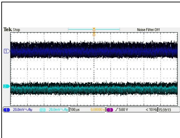
Figure 99: AEE01BB48-M Ripple and Noise Measurement Vin = 48Vdc Load: Io = ±0.625A Ta = 25°C Ch 1: Vo1 Ch 2: Vo2
