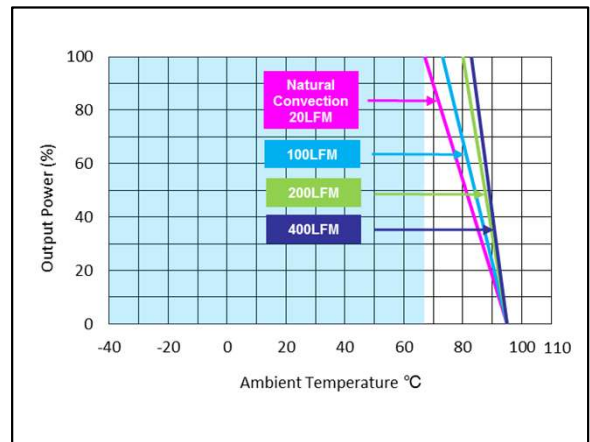
Figure 84: AEE01B48-M Derating Curve (without heatsink). Vin = 48Vdc Load: Io = 0 to 1.25A Ta = 25°C
