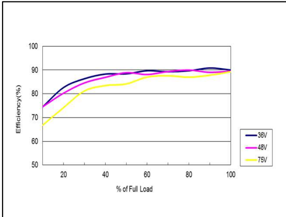
Figure 73: AEE03A48-M Efficiency Versus Output Current Curve Vin = 36 to 75Vdc Load: Io = 0 to 3A Ta = 25°C
