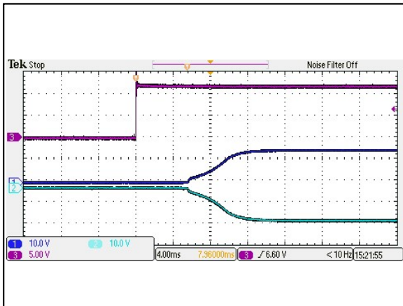
Figure 35: AEE01CC12-M Output Voltage Startup Characteristic by Vin Vin = 12Vdc Load: Io = ±0.5A Ta = 25°C Ch 1: Vo1 Ch 2: Vo2 Ch 3: Vin
