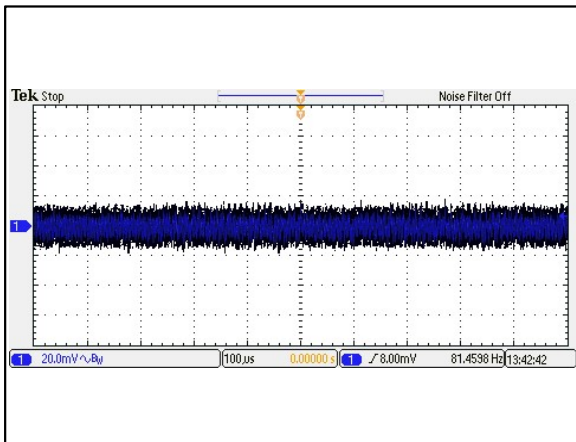
Figure 3: AEE03A12-M Ripple and Noise Measurement Vin = 12Vdc Load: Io = 3A Ta = 25°C Ch 1: Vo
