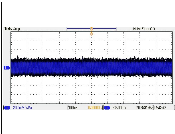
Figure 15: AEE01C12-M Ripple and Noise Measurement Vin = 12Vdc Load: Io = 1A Ta = 25°C Ch 1: Vo
