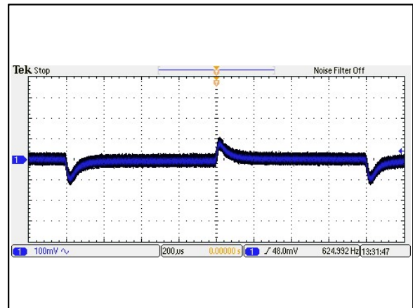
Figure 76: AEE03A48-M Transient Response Vin = 48Vdc Load: Io = 100% to 75% load change Ta = 25°C Ch 1: Vo
