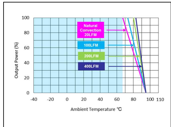
Figure 78: AEE03A48-M Derating Curve (without heatsink). Vin = 48Vdc Load: Io = 0 to 3A Ta = 25°C
