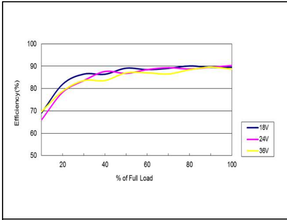
Figure 37: AEE03A24-M Efficiency Versus Output Current Curve Vin = 18 to 36Vdc Load: Io = 0 to 3A Ta = 25°C
