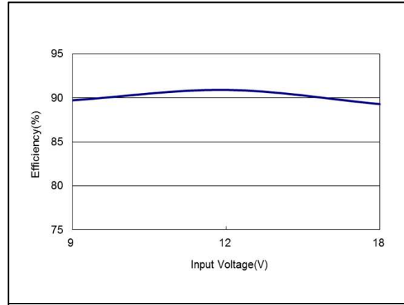
Figure 26: AEE01BB12-M Efficiency Versus Input Voltage Curve Vin = 9 to 18Vdc Load: Io = ±0.625A Ta = 25°C
