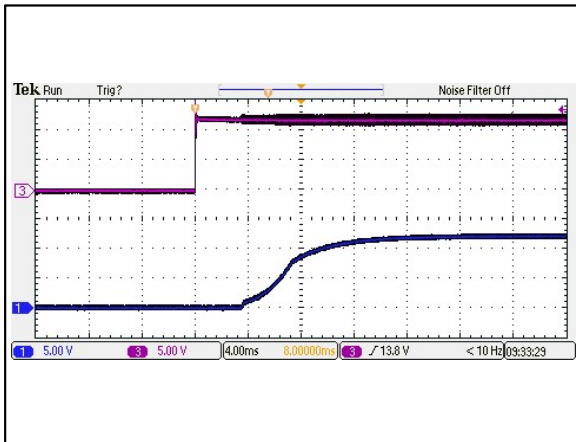
Figure 11: AEE01B12-M Output Voltage Startup Characteristic by Vin Vin = 12Vdc Load: Io = 1.25A Ta = 25°C Ch 1: Vo Ch 3: Vin
