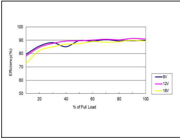
Figure 25: AEE01BB12-M Efficiency Versus Output Current Curve Vin = 9 to 18Vdc Load: Io = 0 to ±0.625A Ta = 25°C
