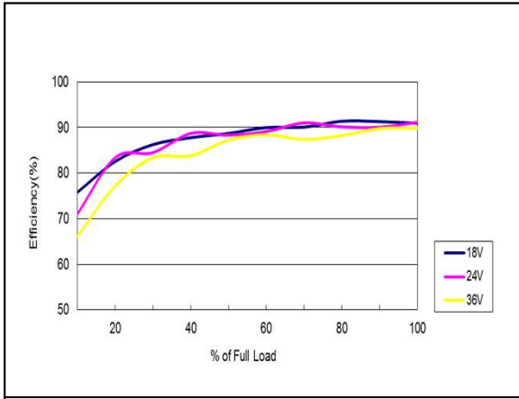
Figure 67: AEE01CC24-M Efficiency Versus Output Current Curve Vin = 18 to 36Vdc Load: Io = 0 to ±0.5A Ta = 25°C
