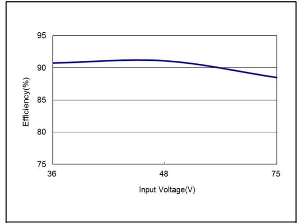
Figure 98: AEE01BB48-M Efficiency Versus Input Voltage Curve Vin = 36 to 75Vdc Load: Io = ±0.625A Ta = 25°C
