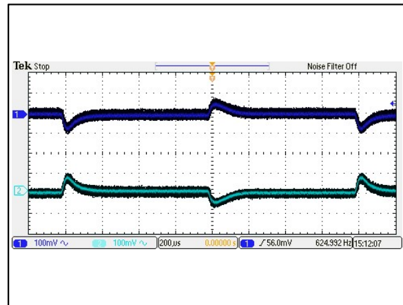
Figure 70: AEE01CC24-M Transient Response Vin = 24Vdc Load: Io = 100% to 75% load change Ta = 25°C Ch 1: Vo1 Ch 2: Vo2
