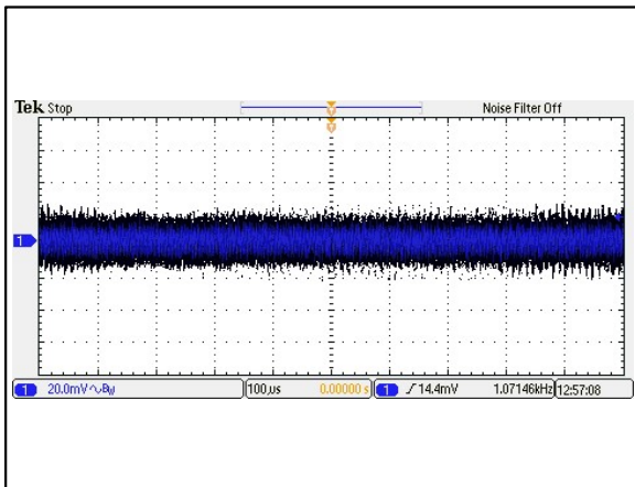
Figure 87: AEE01C48-M Ripple and Noise Measurement Vin = 48Vdc Load: Io = 1A Ta = 25°C Ch 1: Vo
