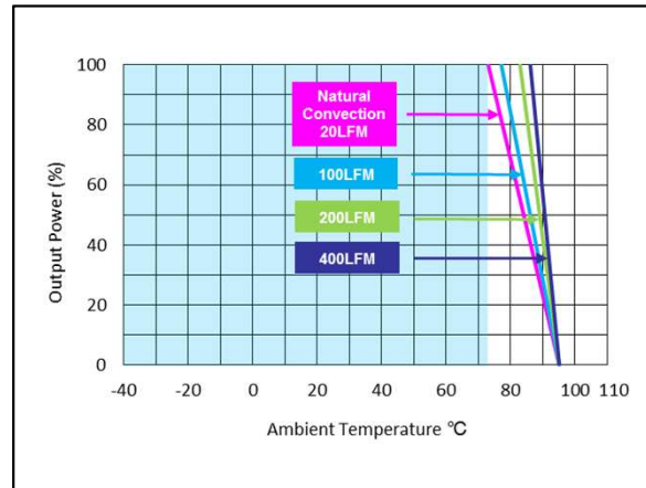
Figure 60: AEE01H24-M Derating Curve (without heatsink). Vin = 24Vdc Load: Io = 0 to 0.625A Ta = 25°C
