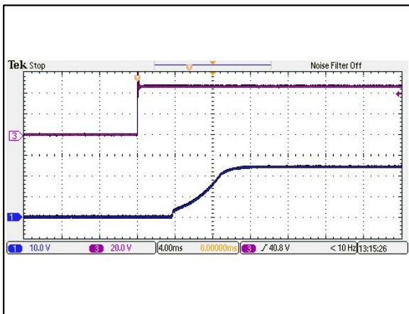
Figure 95: AEE01H48-M Output Voltage Startup Characteristic by Vin Vin = 48Vdc Load: Io = 0.625A Ta = 25°C Ch 1: Vo Ch 3: Vin
