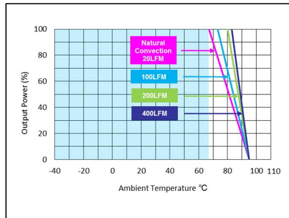
Figure 24: AEE01H12-M Derating Curve (without heatsink). Vin = 12Vdc Load: Io = 0 to 0.625A Ta = 25°C
