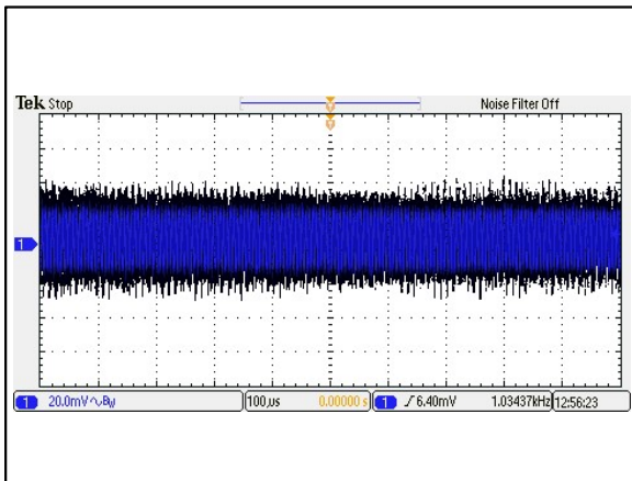
Figure 51: AEE01C24-M Ripple and Noise Measurement Vin = 24Vdc Load: Io = 1A Ta = 25°C Ch 1: Vo
