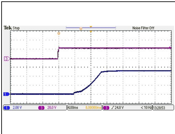
Figure 41: AEE03A24-M Output Voltage Startup Characteristic by Vin Vin = 24Vdc Load: Io = 3A Ta = 25°C Ch 1: Vo Ch 3: Vin
