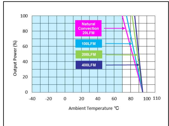
Figure 102: AEE01BB48-M Derating Curve (without heatsink). Vin = 48Vdc Load: Io = 0 to ±0.625A Ta = 25°C
