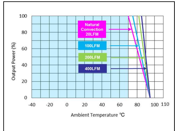
Figure 48: AEE01B24-M Derating Curve (without heatsink). Vin = 24Vdc Load: Io = 0 to 1.25A Ta = 25°C
