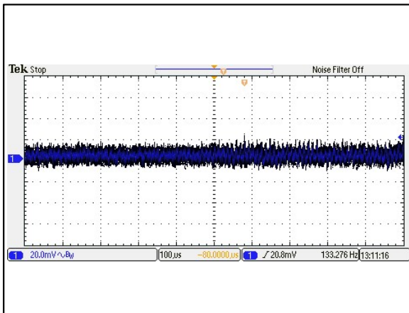
Figure 21: AEE01H12-M Ripple and Noise Measurement Vin = 12Vdc Load: Io = 0.625A Ta = 25°C Ch 1: Vo
