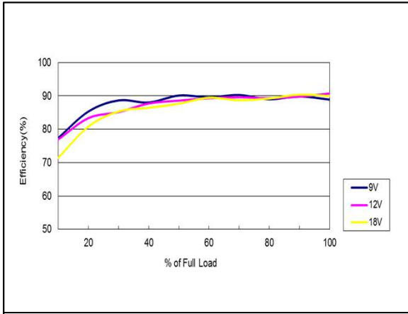
Figure 31: AEE01CC12-M Efficiency Versus Output Current Curve Vin = 9 to 18Vdc Load: Io = 0 to ±0.5A Ta = 25°C
