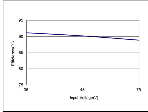
Figure 92: AEE01H48-M Efficiency Versus Input Voltage Curve Vin = 36 to 75Vdc Load: Io = 0.625A Ta = 25°C
