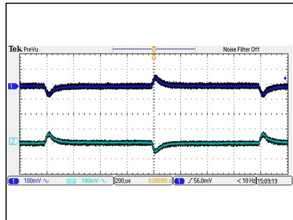
Figure 28: AEE01BB12-M Transient Response Vin = 12Vdc Load: Io = 100% to 75% load change Ta = 25°C Ch 1: Vo1 Ch 2: Vo2
