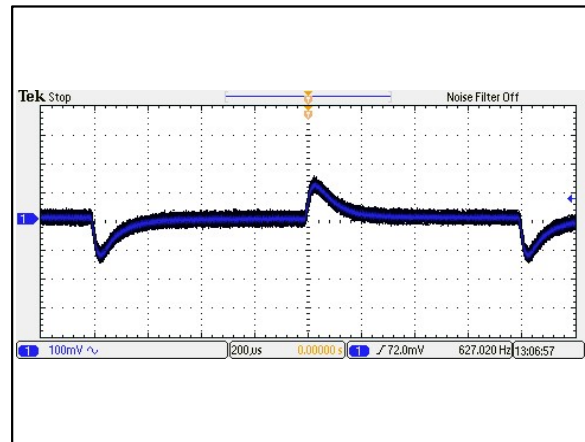
Figure 94: AEE01H48-M Transient Response Vin = 48Vdc Load: Io = 100% to 75% load change Ta = 25°C Ch 1: Vo
