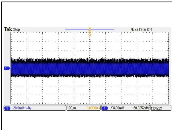
Figure 75: AEE03A48-M Ripple and Noise Measurement Vin = 48Vdc Load: Io = 3A Ta = 25°C Ch 1: Vo
