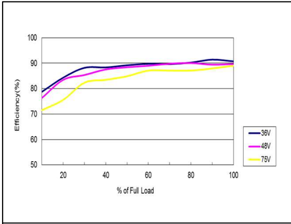
Figure 79: AEE01B48-M Efficiency Versus Output Current Curve Vin = 36 to 75Vdc Load: Io = 0 to 1.25A Ta = 25°C
