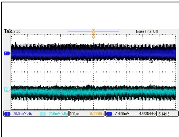
Figure 69: AEE01CC24-M Ripple and Noise Measurement Vin = 24Vdc Load: Io = ±0.5A Ta = 25°C Ch 1: Vo1 Ch 2: Vo2
