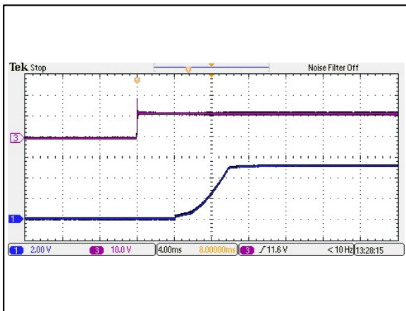
Figure 5: AEE03A12-M Output Voltage Startup Characteristic by Vin Vin = 12Vdc Load: Io = 3A Ta = 25°C Ch 1: Vo Ch 3: Vin
