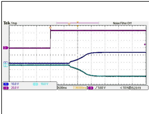
Figure 107: AEE01CC48-M Output Voltage Startup Characteristic by Vin Vin = 48Vdc Load: Io = ±0.5A Ta = 25°C Ch 1: Vo1 Ch 2: Vo2 Ch 3: Vin
