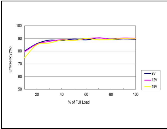
Figure 19: AEE01H12-M Efficiency Versus Output Current Curve Vin = 9 to 18Vdc Load: Io = 0 to 0.625A Ta = 25°C
