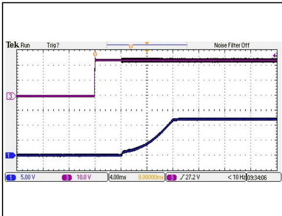
Figure 47: AEE01B24-M Output Voltage Startup Characteristic by Vin Vin = 24Vdc Load: Io = 1.25A Ta = 25°C Ch 1: Vo Ch 3: Vin
