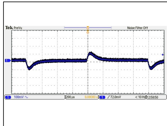
Figure 88: AEE01C48-M Transient Response Vin = 48Vdc Load: Io = 100% to 75% load change Ta = 25°C Ch 1: Vo
