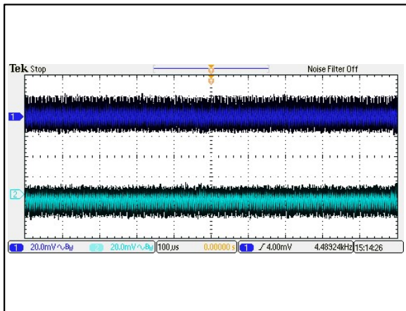
Figure 105: AEE01CC48-M Ripple and Noise Measurement Vin = 48Vdc Load: Io = ±0.5A Ta = 25°C Ch 1: Vo1 Ch 2: Vo2
