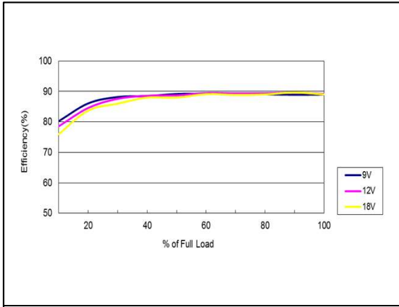
Figure 13: AEE01C12-M Efficiency Versus Output Current Curve Vin = 9 to 18Vdc Load: Io = 0 to 1A Ta = 25°C
