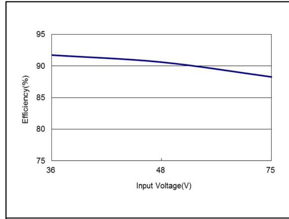
Figure 86: AEE01C48-M Efficiency Versus Input Voltage Curve Vin = 36 to 75Vdc Load: Io = 1A Ta = 25°C
