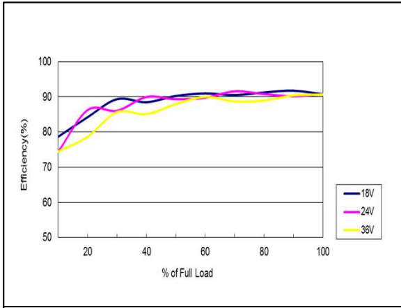
Figure 55: AEE01H24-M Efficiency Versus Output Current Curve Vin = 18 to 36Vdc Load: Io = 0 to 0.625A Ta = 25°C
