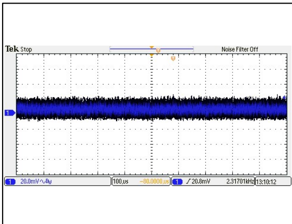
Figure 93: AEE01H48-M Ripple and Noise Measurement Vin = 48Vdc Load: Io = 0.625A Ta = 25°C Ch 1: Vo
