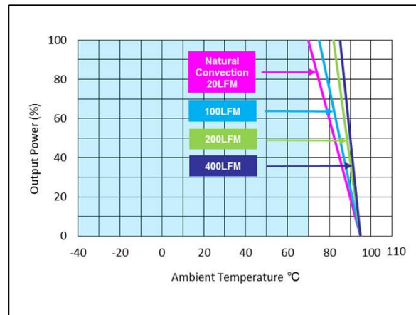
Figure 72: AEE01CC24-M Derating Curve (without heatsink). Vin = 24Vdc Load: Io = 0 to ±0.5A Ta = 25°C
